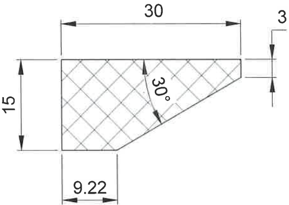
DETAIL 3: GASKET (SECTION)
