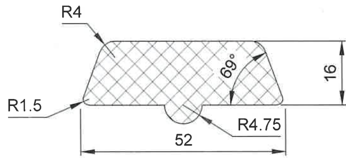
DETAIL 2: GASKET (SECTION)
