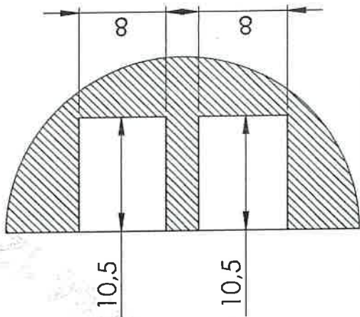
DETAIL D SCALE 2:1
