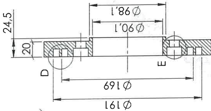
SECTION C-C SCALE 1:3
