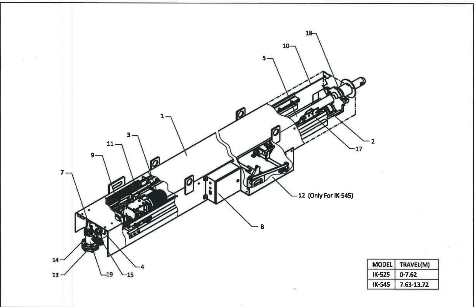
Figure 3.3 IK-525/545 Sootblower Installation
